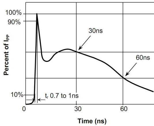
Fig.1 Pulse Waveform-ESD(IEC61000-4-2)
