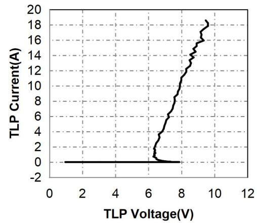
Fig.2 Transmission Line Pulse (TLP)
