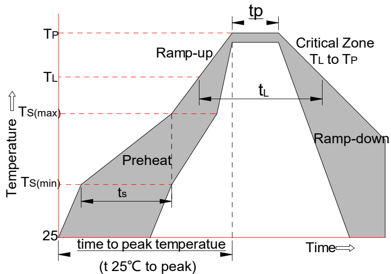
FIG.5: Reflow condition
