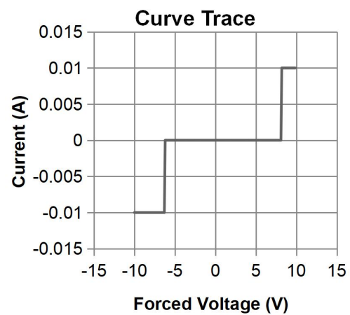
Fig.4 IV Curve
