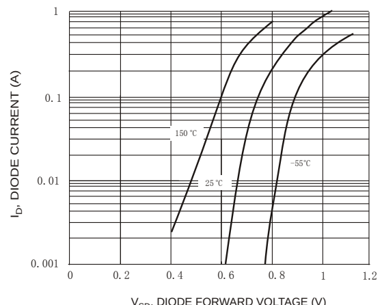
Fig. 6 Body Diode Current vs. Body Diode Voltage
