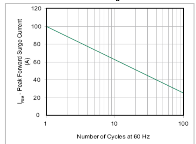
Figure 6 – Maximum Non-Repetitive Forward Surge Current
