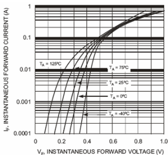
Fig. 1 Forward Characteristics
