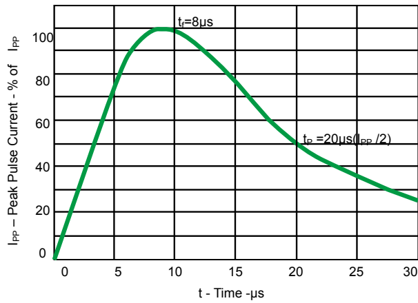
Fig 1. Pulse Waveform
