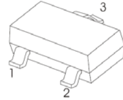
SOT-323 1. BASE 2. EMITTER 3. COLLECTOR
