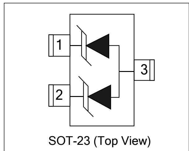
Schematic & PIN Configuratio
