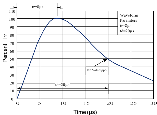
Figure 5: Pulse Waveform
