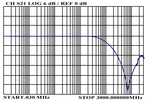
Figure 2: Insertion Loss
